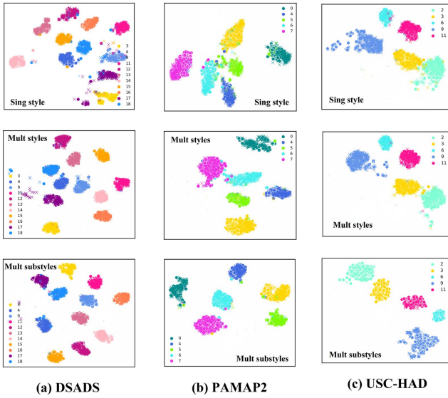
Fig. 4. T-SNE visualization of DSADS, PAMAP2, USC-HAD datasets. The original and synthetic data are represented by shapes dots and crosses, and each class is denoted by a color. Best viewed in color and zoom in.
