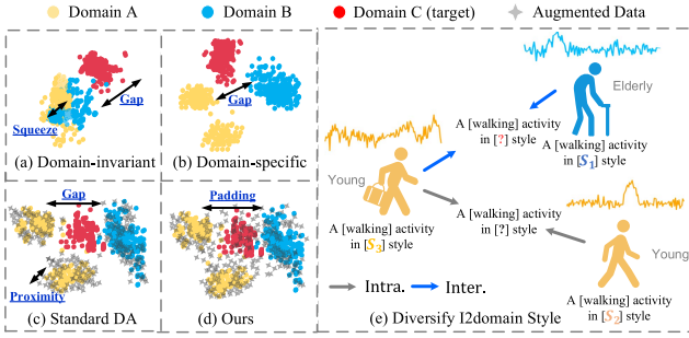
Fig. 1. T-SNE visualization of time-series activity features extracted by various methods across three domains in sensor-based HAR. Existing representation learning methods result in domain gaps as in both (a) and (b), covering a small portion of the target domain (red circles). Standard data augmentation (DA) leads to augmented data (stars), with source domains (orange/blue circles) remaining in close proximity to each other and failing to fill gaps. Our method (d) creates a comprehensive feature space by padding domain gaps via the idea of (e).
