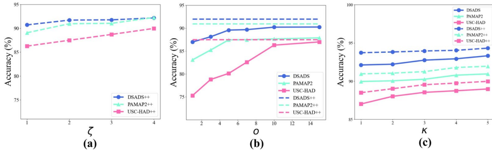
Fig. 8. Hyperparameter sensitivity analysis for DI2SDiff (solid line) and DI2SDiff++ (dashed line): (a) \zeta (b) o (c) \kappa .
