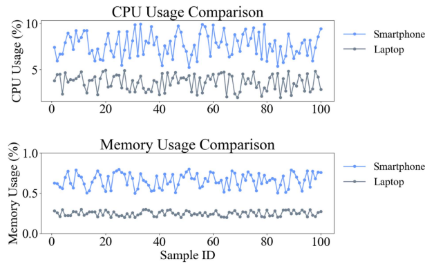
Fig. 12. Performance overhead analysis of DI2SDiff++ on edge devices in terms of CPU usage (%) and memory usage (%) across both smartphone and laptop platforms.
