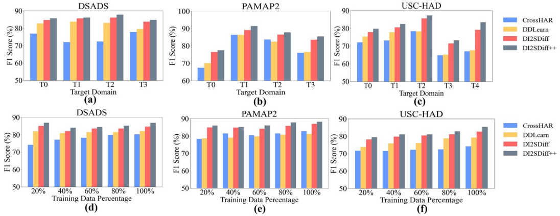
Fig. 6. F1 score (%) comparison of four competitive methods (CrossHAR, DDLearn, DI2SDiff, and DI2SDiff++) on three datasets. Subfigures (a–c) show the results with 20% training data across different target domains; subfigures (d–f) show performance under varying training data percentages.
