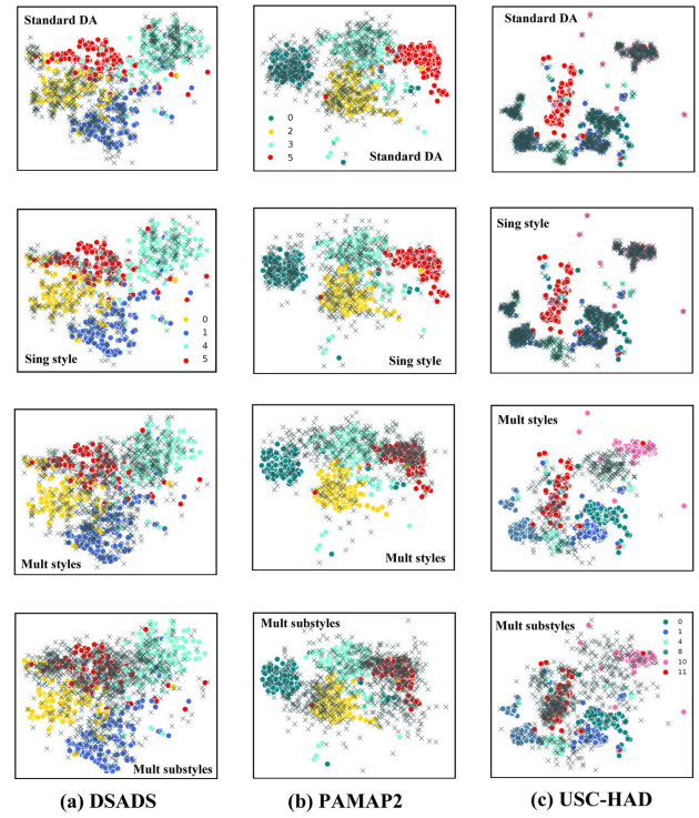
Fig. 5. T-SNE visualization of DSADS, PAMAP2, and USC-HAD datasets. Each domain category is represented by a color, and the target domain is represented by a red dot. The original and synthetic data are represented by shapes dots and crosses, respectively. Best viewed in color and zoom in.
