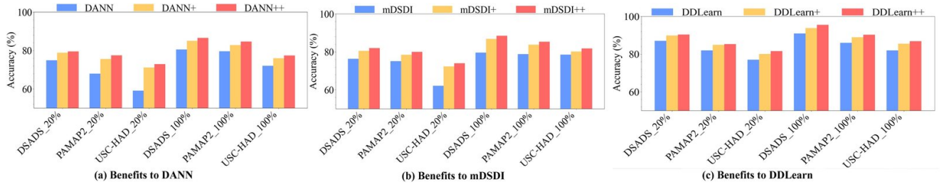
Fig. 10. Enhanced performance of (a) DANN [74], (b) mDSDI [20] and (c) DDLearn [14] with DI2SDiff's data generation (+) and DI2SDiff++'s data generation (++) on 20% and 100% training data in three datasets.
