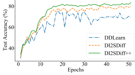
Fig. 9. Trend of test accuracy in comparison as the number of epochs increases on the first tasks of the PAMAP2 dataset with 20% training data.
