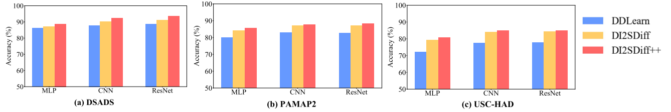
Fig. 11. Results with different backbones on the three datasets.
