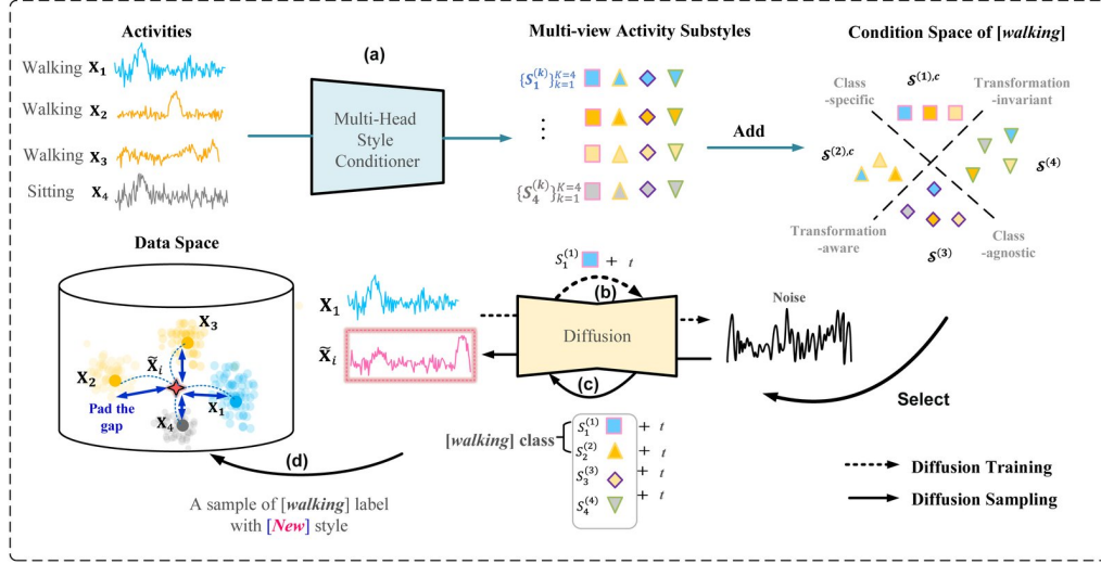
Fig. 3. Illustration of the diffusion within DI2SDiff++. Suppose we have three original walking instances \mathbf{X}_1 , \mathbf{X}_2 , and \mathbf{X}_3 , and a sitting instance \mathbf{X}_4 . Here, \mathbf{X}_1 and \mathbf{X}_4 are from different domains, while \mathbf{X}_2 and \mathbf{X}_3 belong to the same domain. (a) The multi-head style conditioner processes these samples to extract four substyle features, resulting in features such as \{S_1^{(k)}\}_{k=1}^4 for \mathbf{X}_1 . The class-specific substyle features are grouped into S^{(1),c} and S^{(2),c} , while the class-agnostic substyle features are stored in S^{(3)} and S^{(4)} . (b) During training, the diffusion retrieves each data sample (e.g., \mathbf{X}_1 ) along with one substyle component (e.g., S_1^{(1)} ) for the forward process. (c) To generate a walking instance \tilde{\mathbf{X}}_i , style components S_1^{(1)}, S_2^{(2)}, S_3^{(3)}, S_4^{(4)} are selected, originating from the samples \mathbf{X}_1, \mathbf{X}_2, \mathbf{X}_3 , and \mathbf{X}_4 , respectively, to form a new substyle combination. (d) During sampling, the diffusion takes in noise and the substyle combination for the reverse process. (e) The generated sample \tilde{\mathbf{X}}_i enriches the data space by combining four distinct substyles from different samples and domains.
