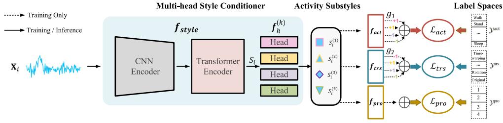
Fig. 2. The multi-head style conditioner of DI2SDiff++. This style conditioner integrates a combination of a CNN and a Transformer encoder ( f_{style} ), followed by four heads f_h^{(k)} . 1) During training, given an activity instance X_i (which can be original data or transformed data), four heads of the style conditioner decompose it into distinct substyle features (different shapes). These substyles are then processed through three fully connected layers ( f_{act} , f_{trs} , f_{pro} ) to execute separate multi-task learning objectives. Each task is optimized via its respective loss function: L_{act} , L_{trs} , and L_{pro} . 2) During inference, only the style conditioner module is used to decompose the original training data into four distinct substyles. The first and second substyles, S_i^{(1)} and S_i^{(2)} , capture class-specific semantics, while the third and fourth substyles, S_i^{(3)} and S_i^{(4)} , represent class-agnostic features.
